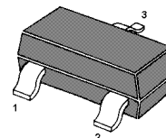
1. Emitter 2. Base 3. Collector SOT-23 Plastic Package
